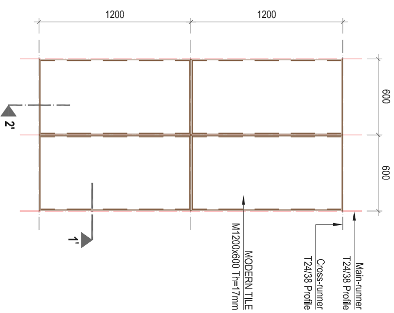
MODULE 1200x600mm
