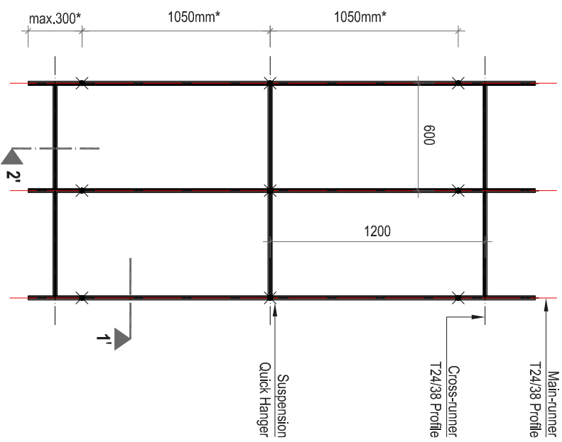
STRUCTURE LAY-OUT scale 1:30
