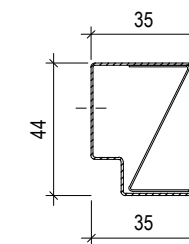
EDGE-PROFILE UW 40 L= max.3000 mm
