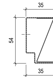
EDGE-PROFILE UW 50 L= max.3000 mm
