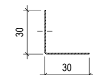
EDGE-PROFILE L 30 L= max.3000 mm
