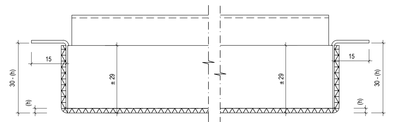
Detail F scale 1:1
