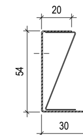
EDGE-PROFILE U 50 L= max.3000 mm
