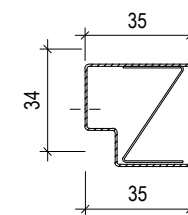
EDGE-PROFILE UW 30 L= max.3000 mm
