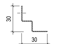
EDGE-PROFILE W 30 L= max.3000 mm
