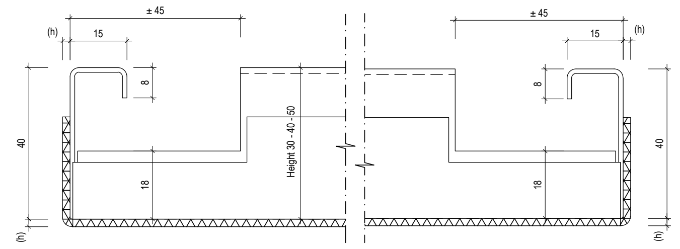
Detail F scale 1:1
