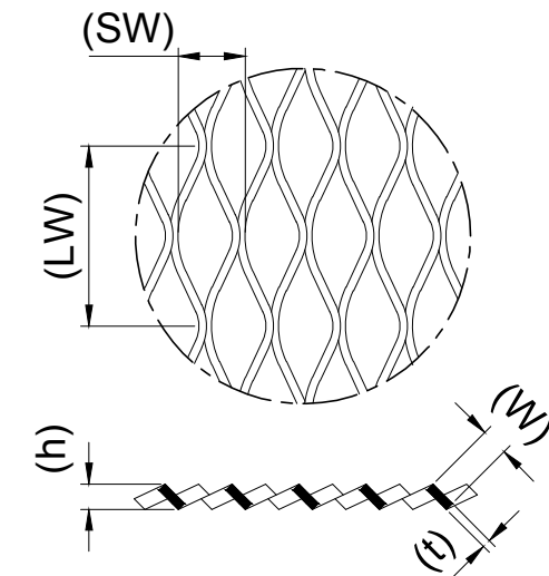
Detail H scale -:- Orientation stretch metal For dimensions see brochure
