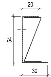
EDGE-PROFILE U 50 L= max.3000 mm
