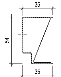
EDGE-PROFILE UW 50 L= max.3000 mm
