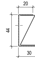
EDGE-PROFILE U 40 L= max.3000 mm
