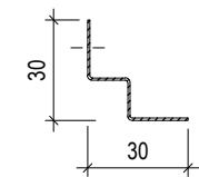
EDGE-PROFILE W 30 L= max.3000 mm
