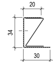
EDGE-PROFILE U 30 L= max.3000 mm
