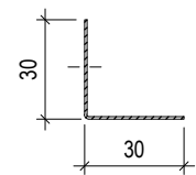
EDGE-PROFILE L 30 L= max.3000 mm
