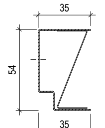
EDGE-PROFILE UW 50 L= max.3000 mm
