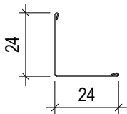
EDGE PROFILE 24x24 mm (non HD) sec
